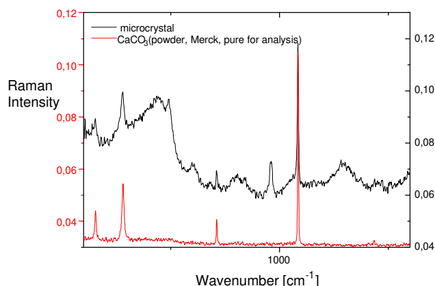
Fig. 2: Raman spectra of pineal gland microcrystal and pure calcite powder.
